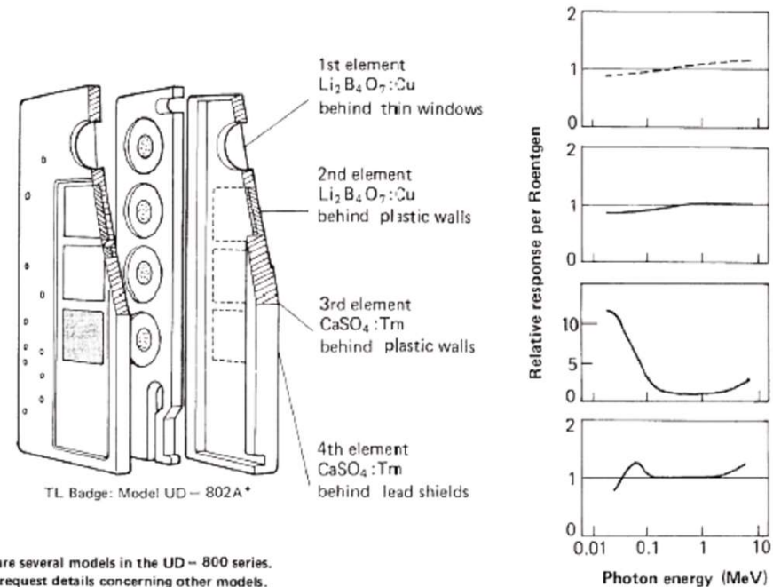
Construction of the model UD-802A, a typical TL badge, and the energy responses of each element.
