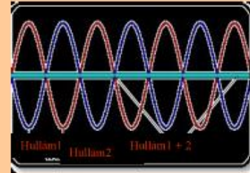
Opposite waves Destructive interference
