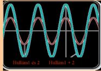
Similar phase Constructive interference
